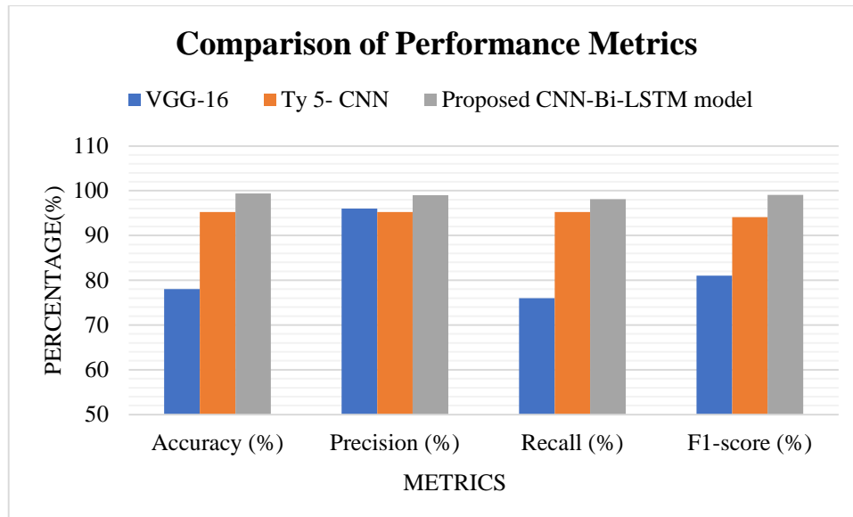
Fig.11. Comparison of Performance Metrics
