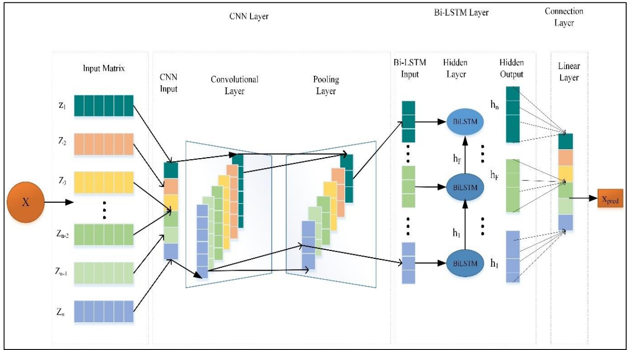
Fig.3. Architecture of Hybrid CNN and Bi-LSTM
